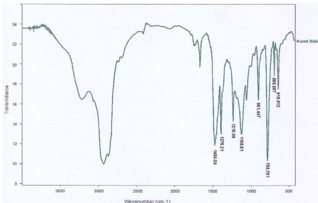
Figure 1. Spectroscopy Analysis of Resiprene 35
